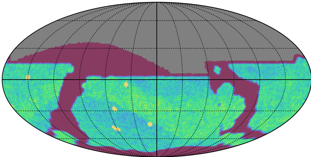
all_long_v3.4_10yrs All sky i band: NVisits
