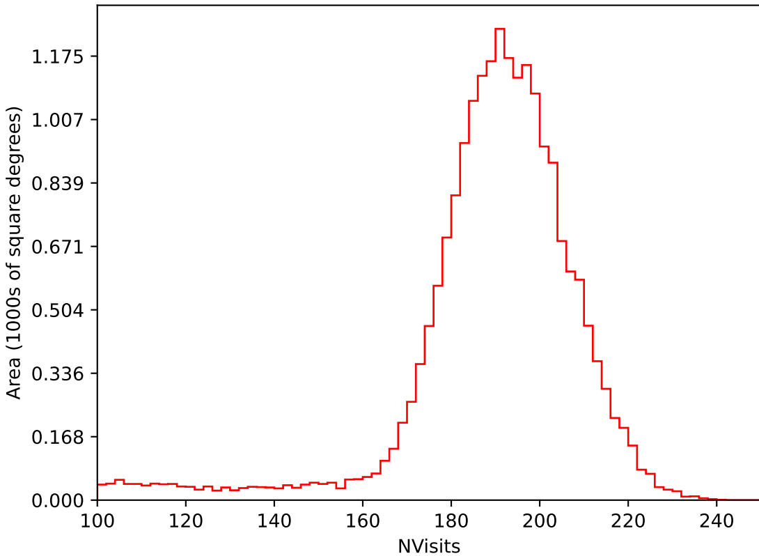
all_long_v3.4_10yrs All sky i band: NVisits
