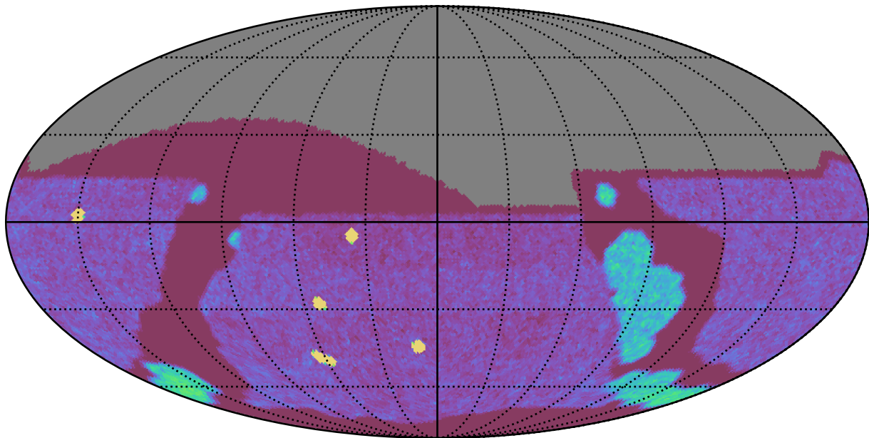
all_long_v3.4_10yrs All sky g band: NVisits
