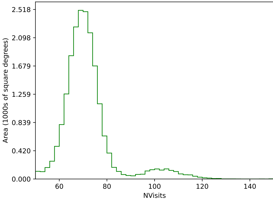
all_long_v3.4_10yrs All sky g band: NVisits
