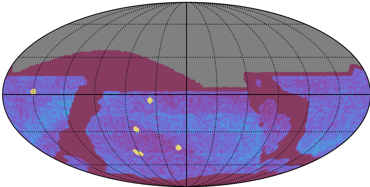
all_long_v3.4_10yrs All sky all bands: NVisits
