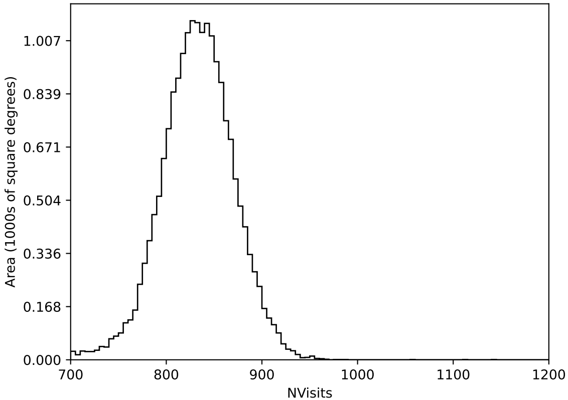
all_long_v3.4_10yrs All sky all bands: NVisits
