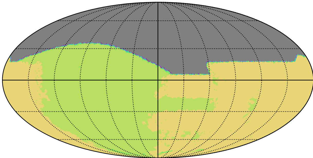
all_long_v3.4_10yrs All sky all bands: NSeasons
