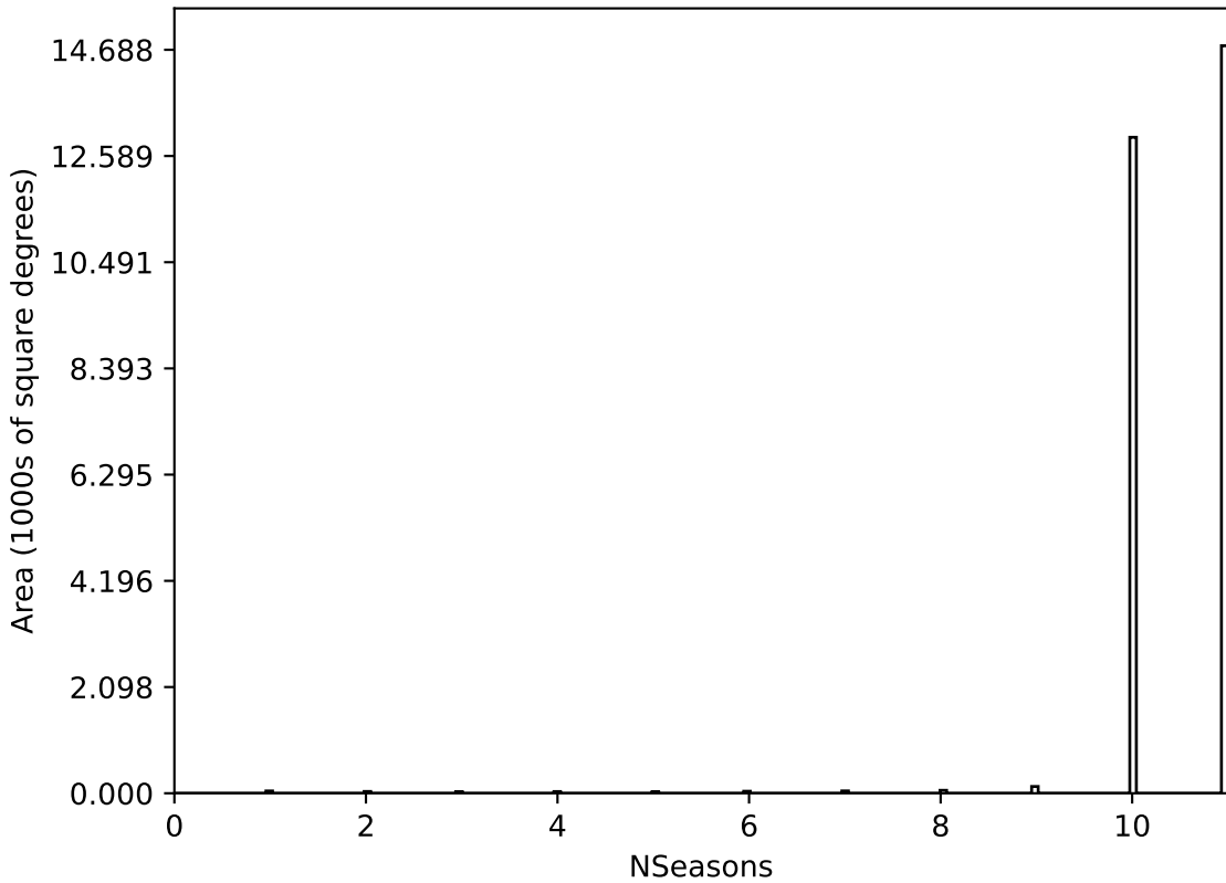
all_long_v3.4_10yrs All sky all bands: NSeasons
