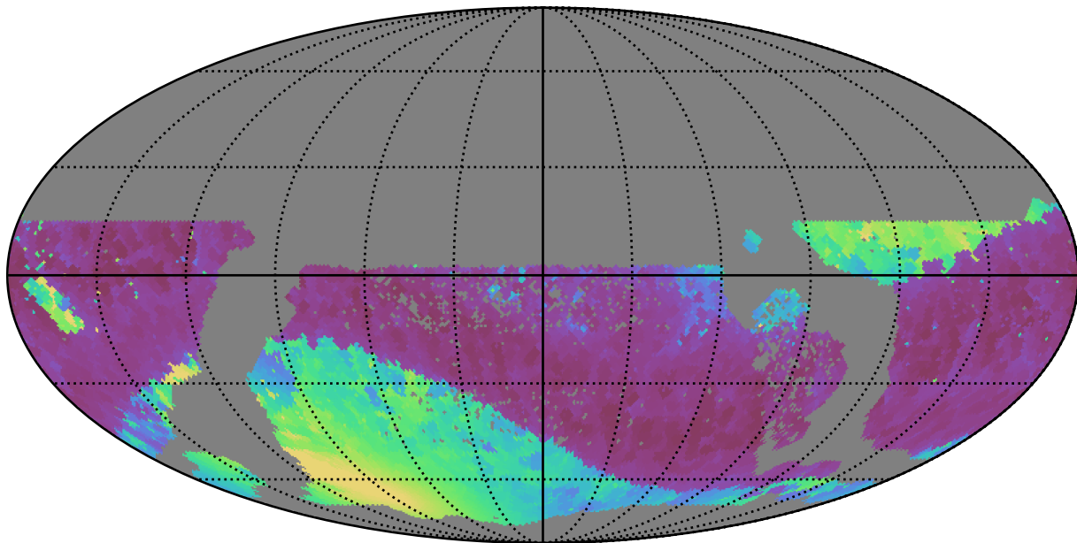
all_long_v3.4_10yrs WFD z band: Min solarElong
