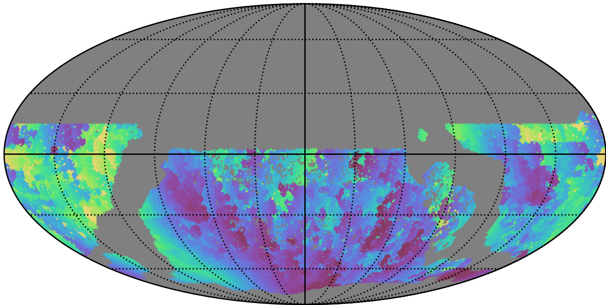
all_long_v3.4_10yrs WFD u band: Min solarElong
