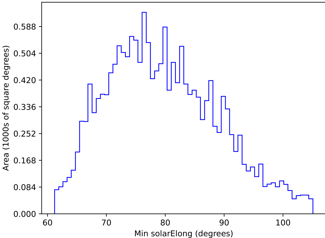
all_long_v3.4_10yrs WFD u band: Min solarElong
