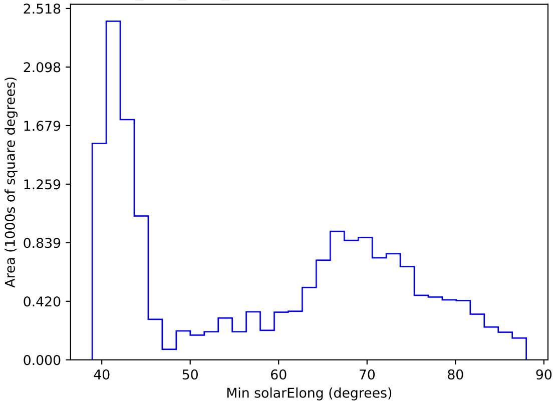
all_long_v3.4_10yrs WFD r band: Min solarElong
