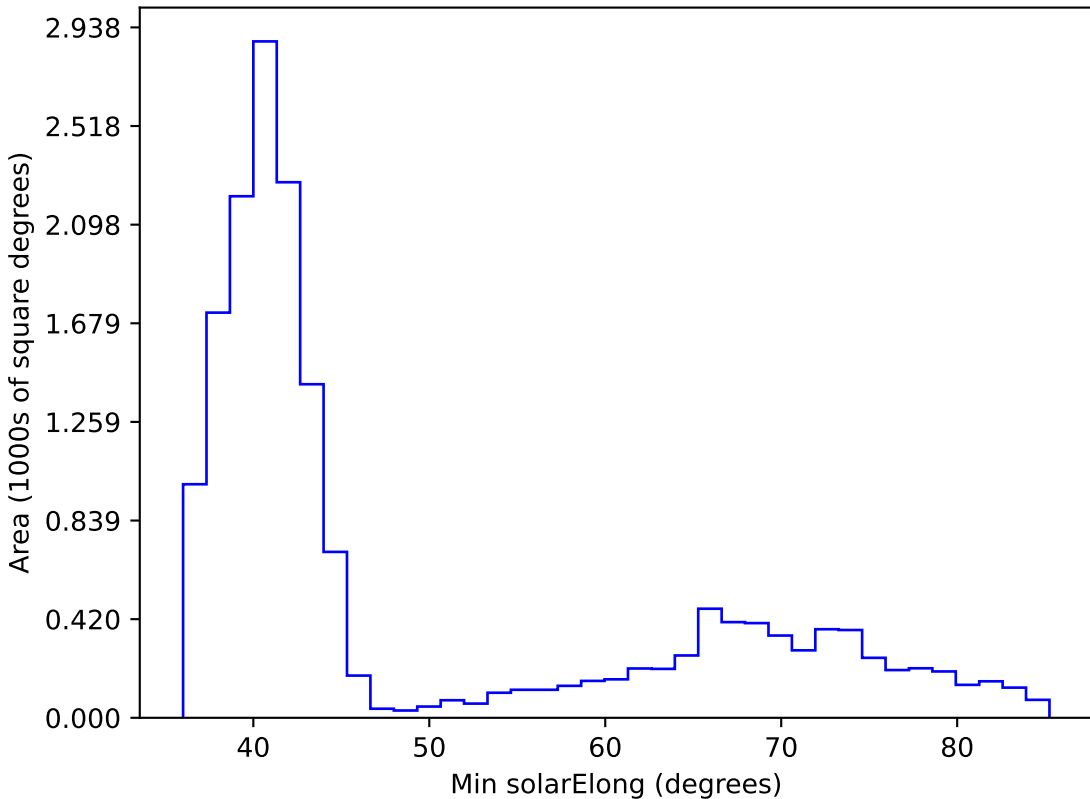
all_long_v3.4_10yrs WFD i band: Min solarElong
