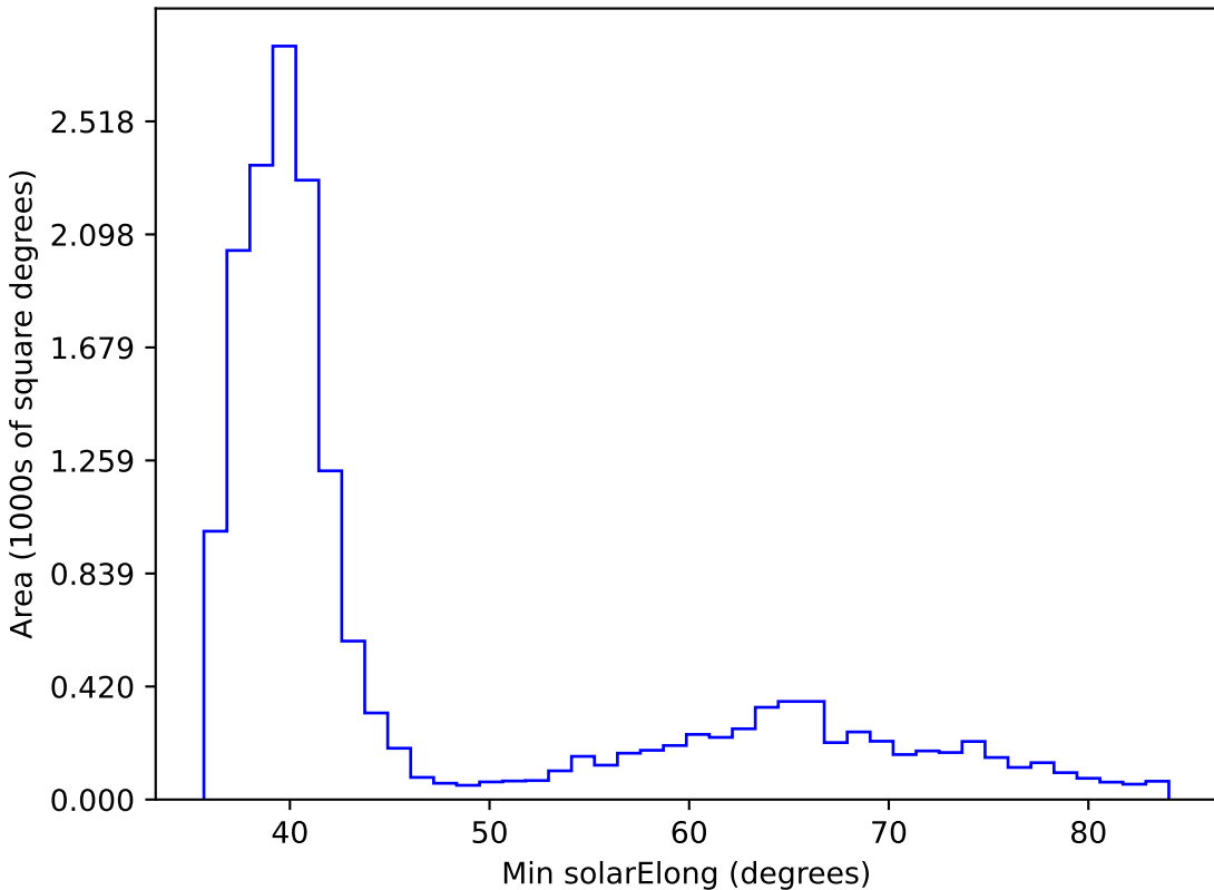
all_long_v3.4_10yrs WFD all bands: Min solarElong
