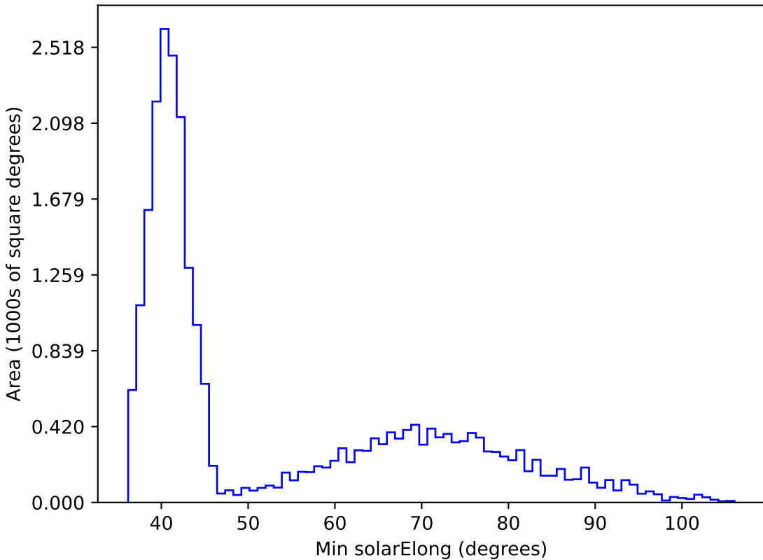
all_long_v3.4_10yrs All sky z band: Min solarElong
