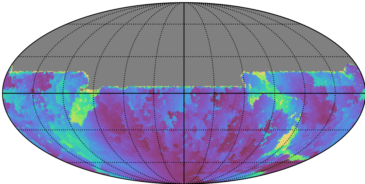
all_long_v3.4_10yrs All sky u band: Min solarElong
