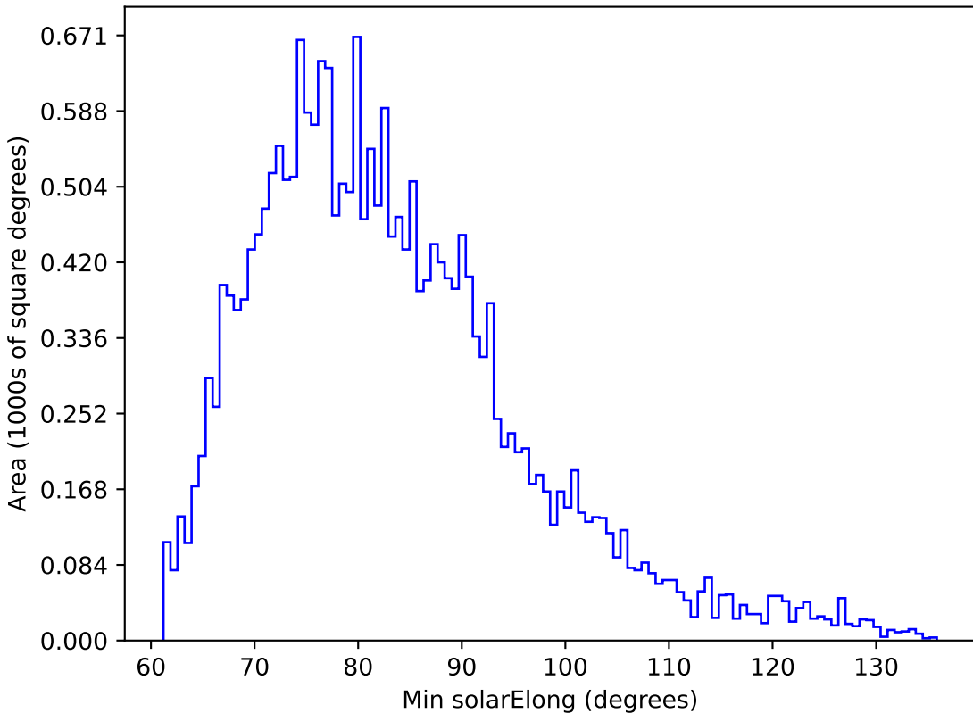
all_long_v3.4_10yrs All sky u band: Min solarElong
