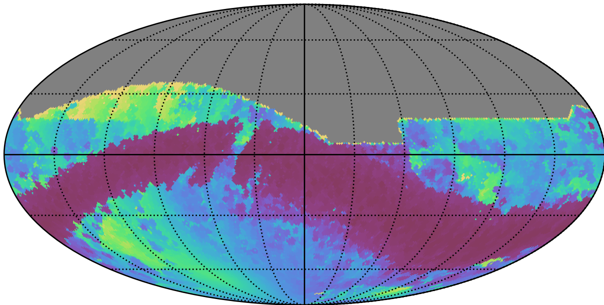
all_long_v3.4_10yrs All sky r band: Min solarElong
