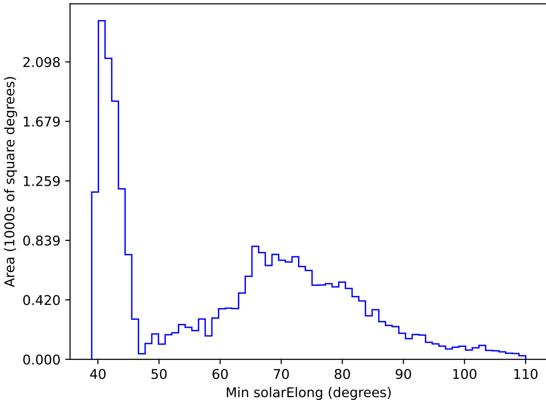
all_long_v3.4_10yrs All sky r band: Min solarElong
