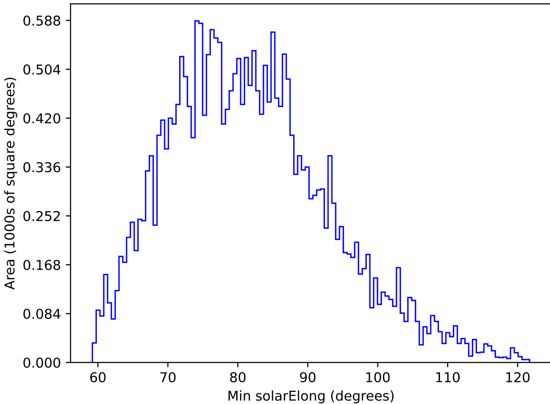
all_long_v3.4_10yrs All sky g band: Min solarElong
