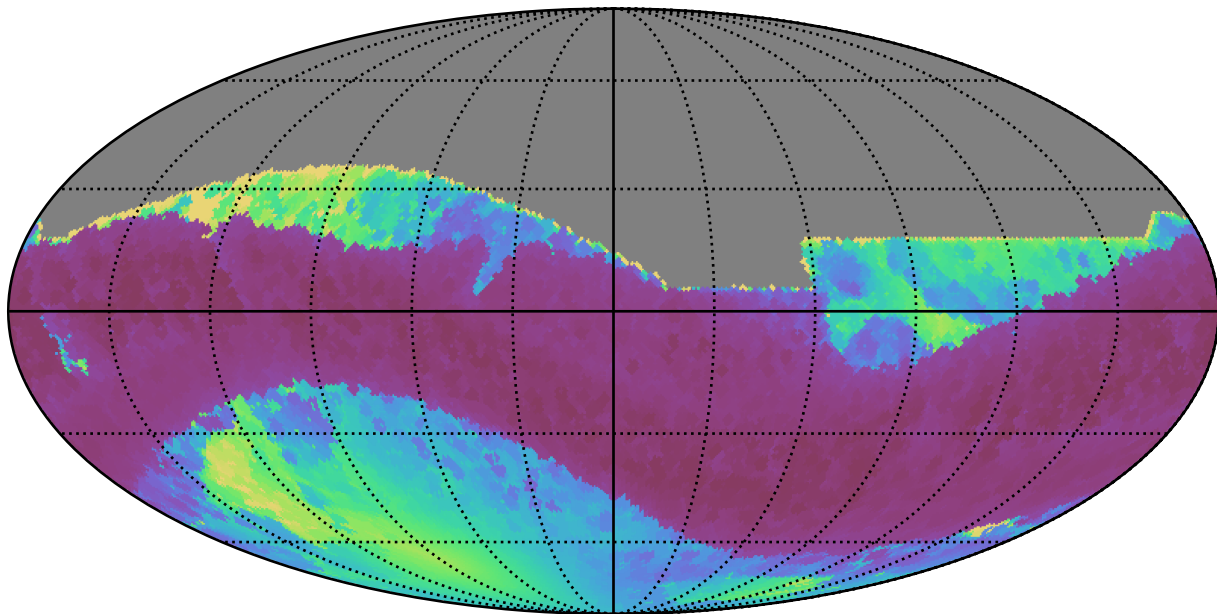
all_long_v3.4_10yrs All sky all bands: Min solarElong
