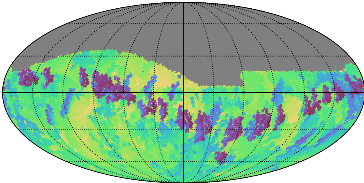
all_long_v3.4_10yrs Yr 1 z band: Min skyBrightness
