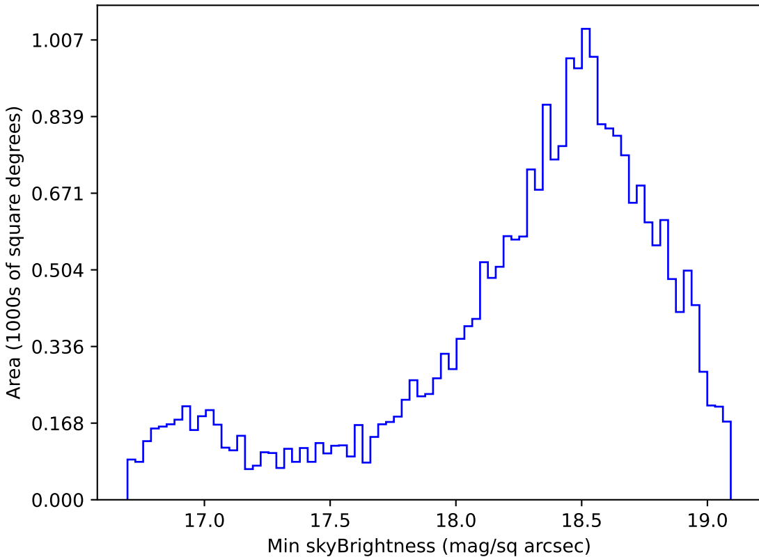
all_long_v3.4_10yrs Yr 1 z band: Min skyBrightness
