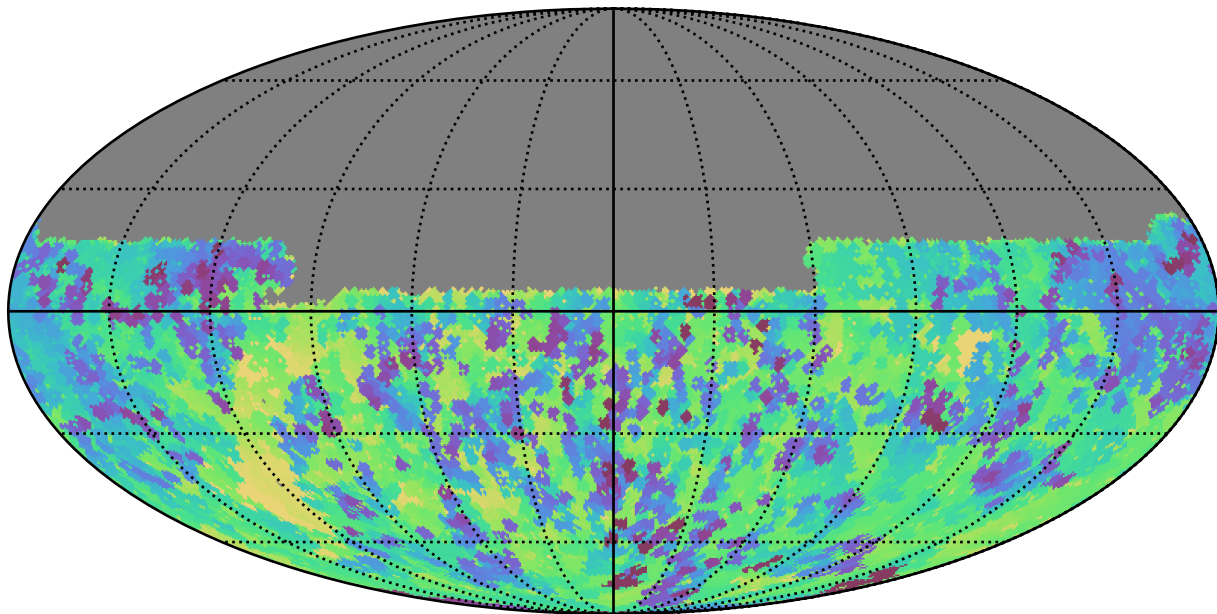
all_long_v3.4_10yrs Yr 1 y band: Min skyBrightness
