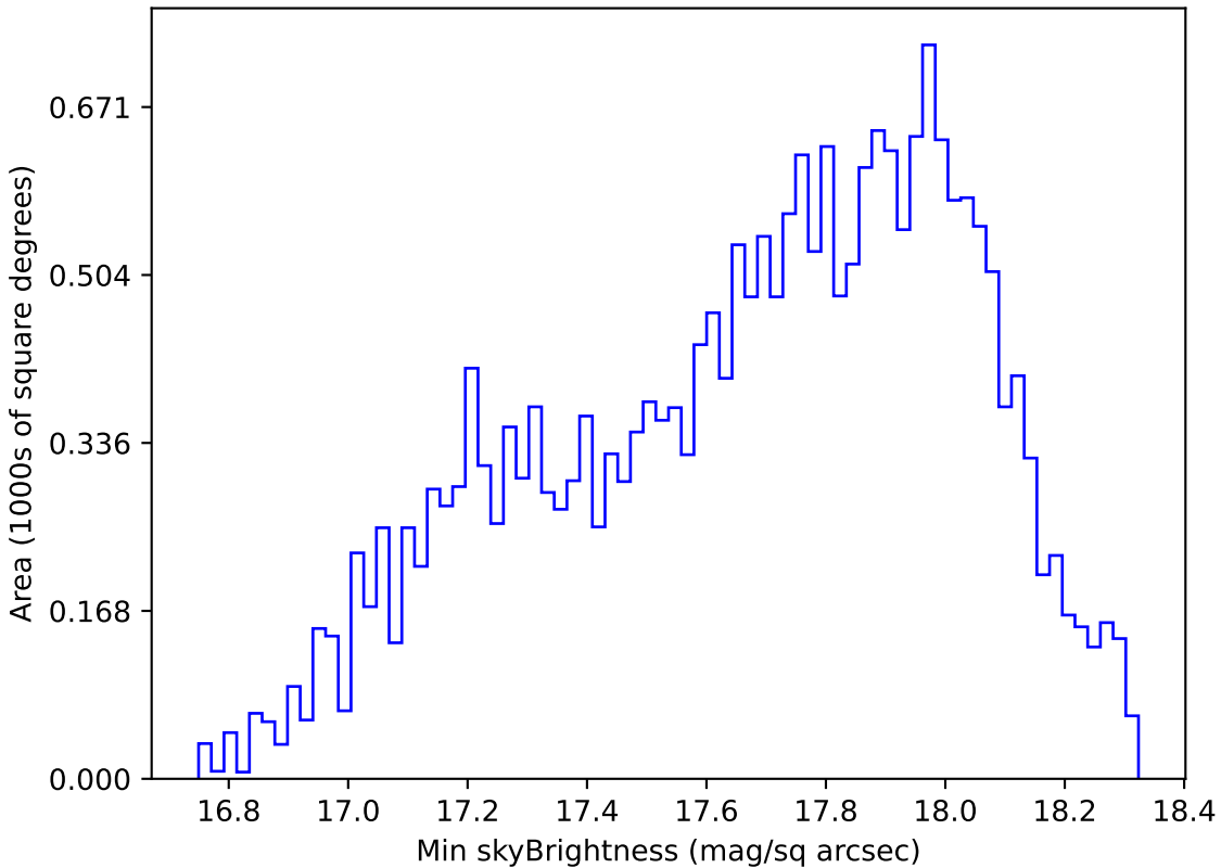
all_long_v3.4_10yrs Yr 1 y band: Min skyBrightness
