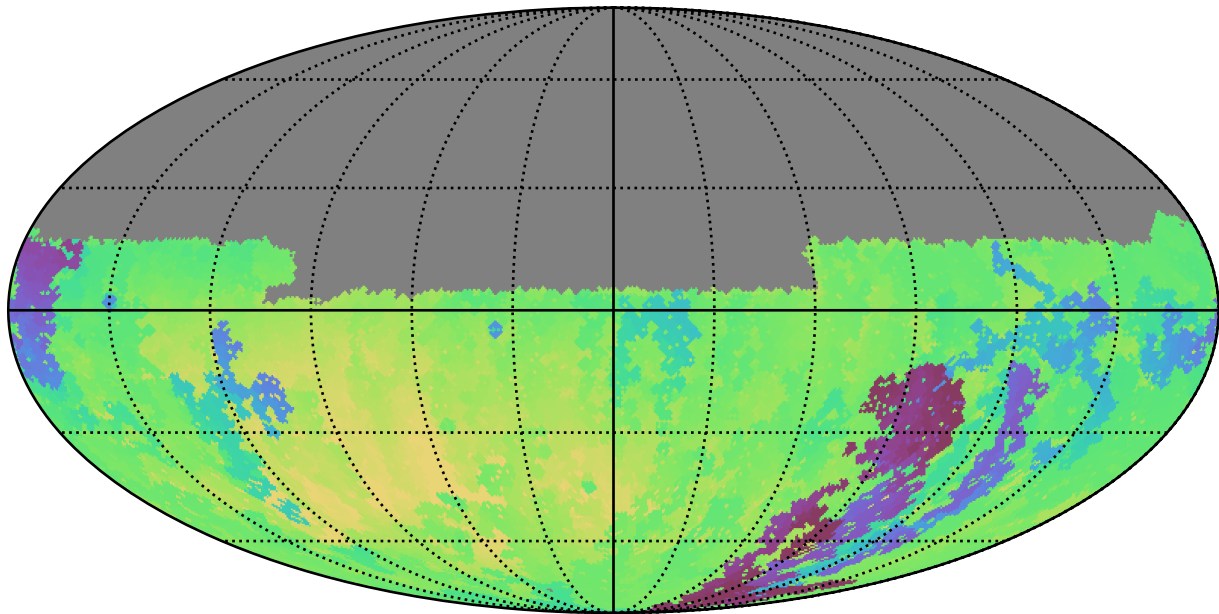
all_long_v3.4_10yrs Yr 1 u band: Min skyBrightness
