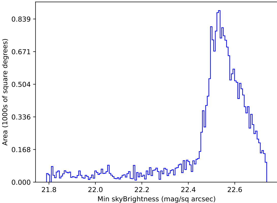
all_long_v3.4_10yrs Yr 1 u band: Min skyBrightness
