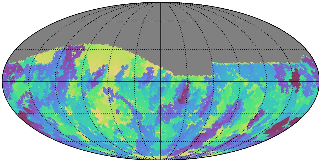
all_long_v3.4_10yrs Yr 1 r band: Min skyBrightness
