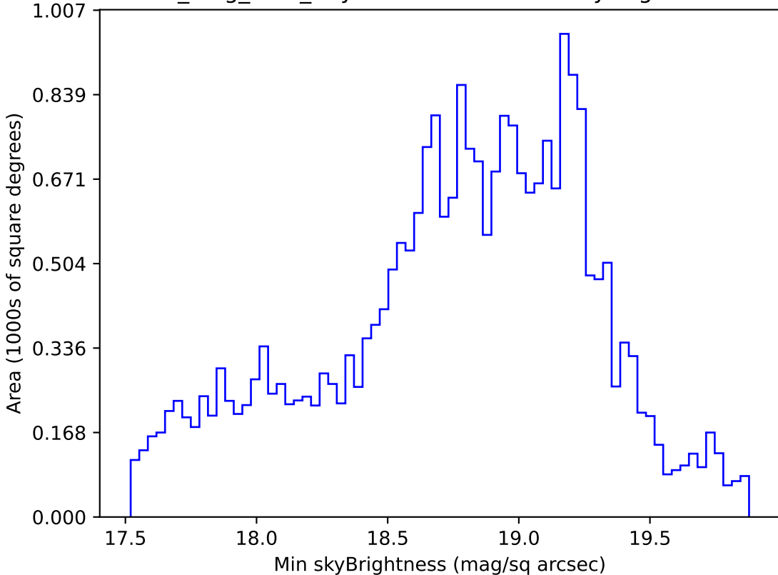
all_long_v3.4_10yrs Yr 1 i band: Min skyBrightness
