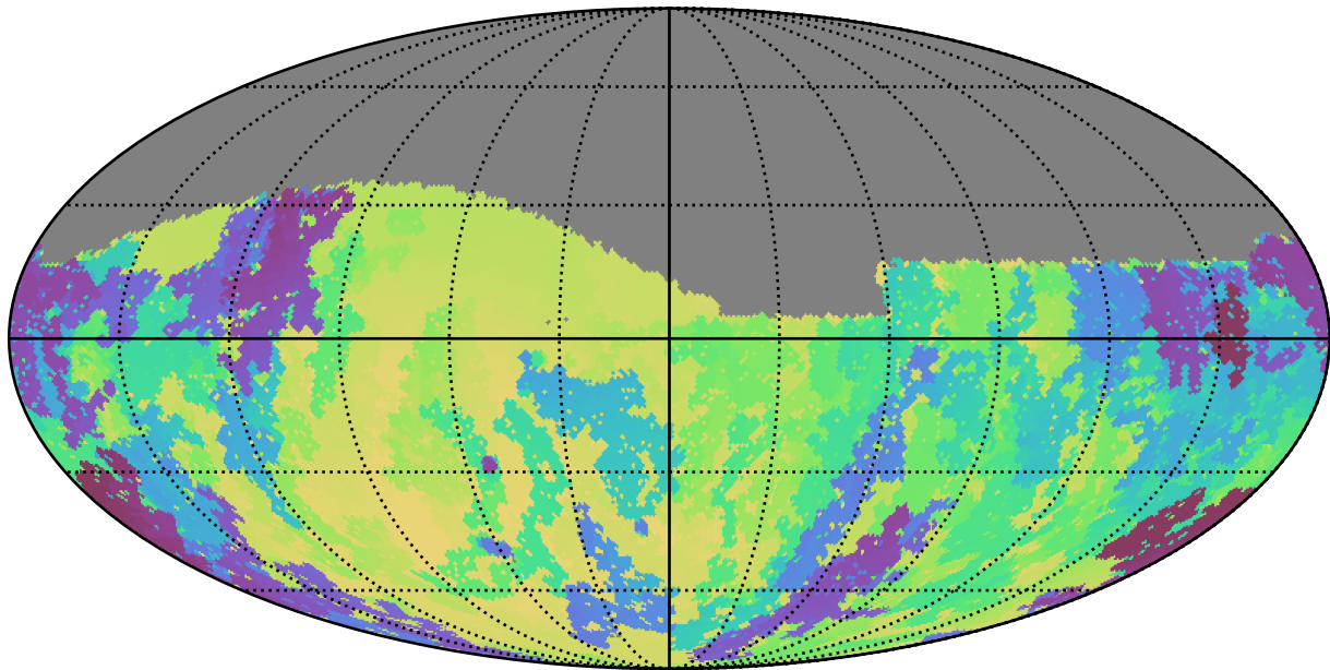
all_long_v3.4_10yrs Yr 1 g band: Min skyBrightness
