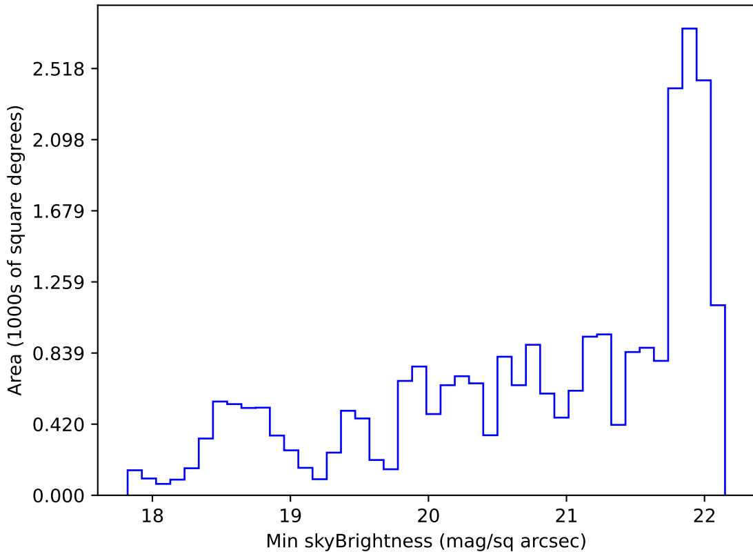
all_long_v3.4_10yrs Yr 1 g band: Min skyBrightness
