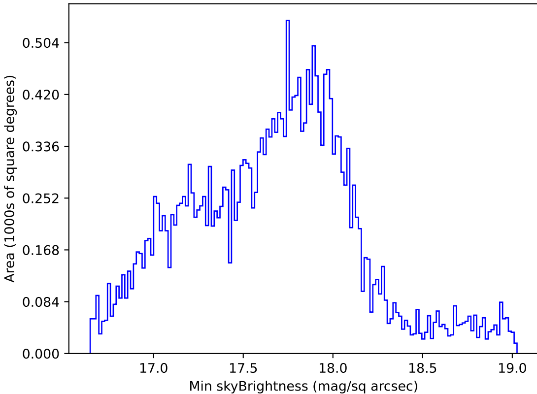
all_long_v3.4_10yrs Yr 1 all bands: Min skyBrightness
