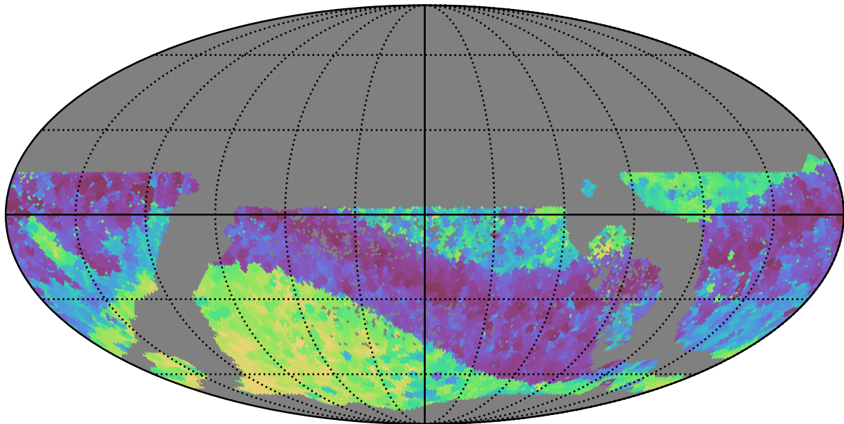
all_long_v3.4_10yrs WFD z band: Min skyBrightness
