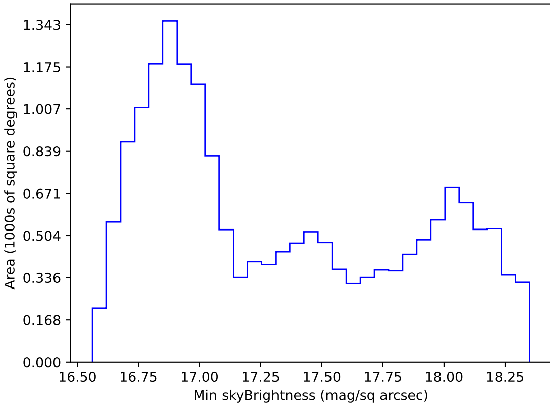
all_long_v3.4_10yrs WFD z band: Min skyBrightness
