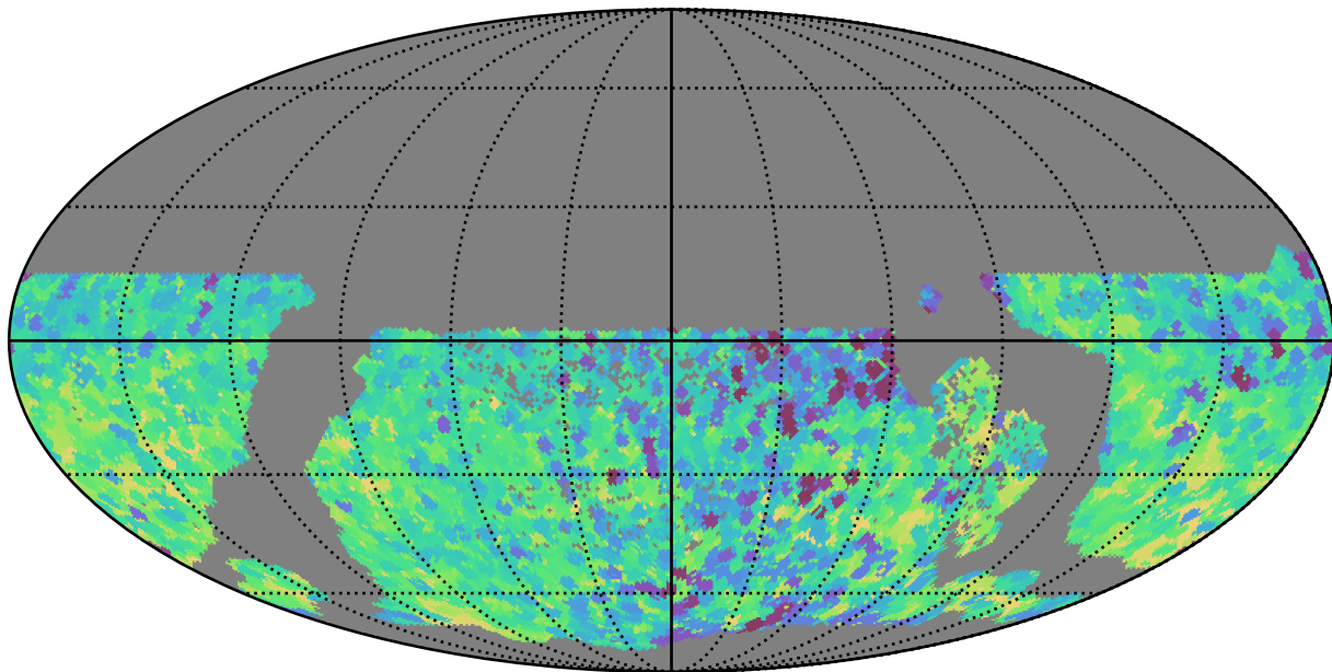
all_long_v3.4_10yrs WFD y band: Min skyBrightness
