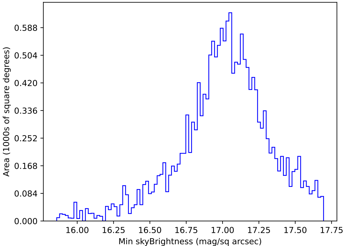
all_long_v3.4_10yrs WFD y band: Min skyBrightness
