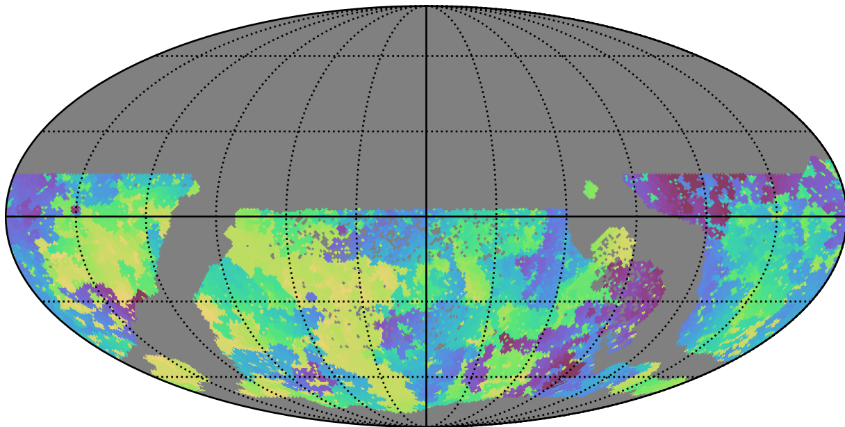
all_long_v3.4_10yrs WFD u band: Min skyBrightness
