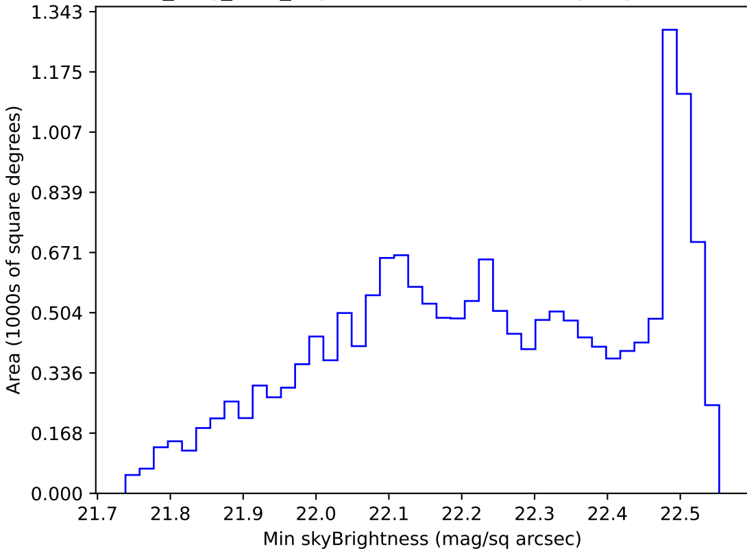
all_long_v3.4_10yrs WFD u band: Min skyBrightness
