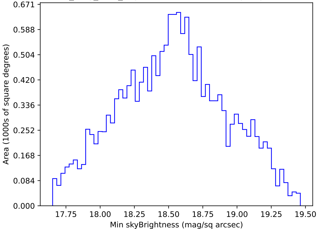
all_long_v3.4_10yrs WFD r band: Min skyBrightness
