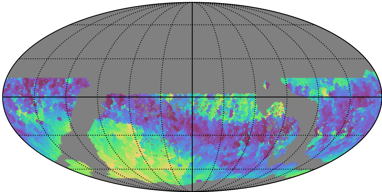
all_long_v3.4_10yrs WFD i band: Min skyBrightness
