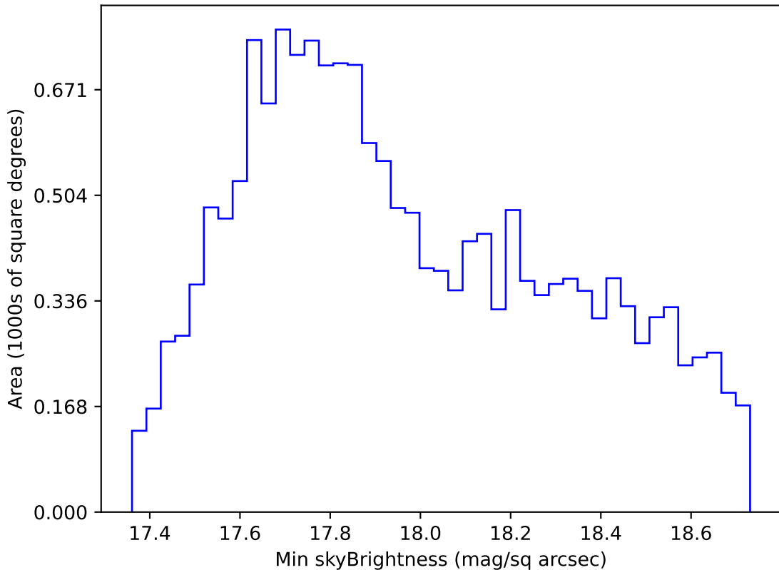
all_long_v3.4_10yrs WFD i band: Min skyBrightness
