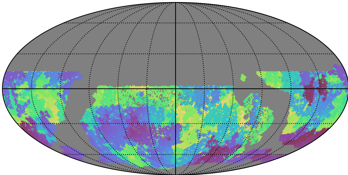
all_long_v3.4_10yrs WFD g band: Min skyBrightness
