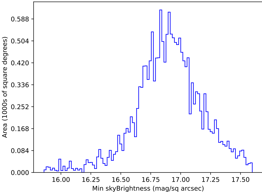
all_long_v3.4_10yrs WFD all bands: Min skyBrightness
