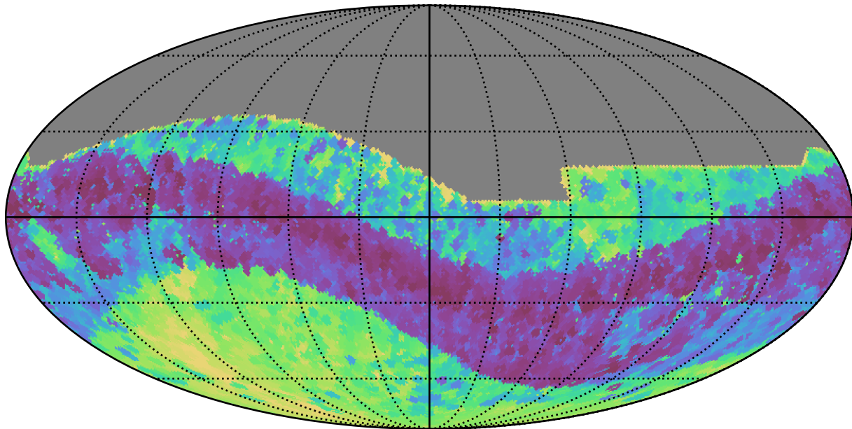
all_long_v3.4_10yrs All sky z band: Min skyBrightness
