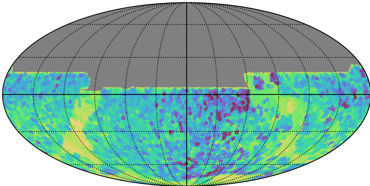
all_long_v3.4_10yrs All sky y band: Min skyBrightness
