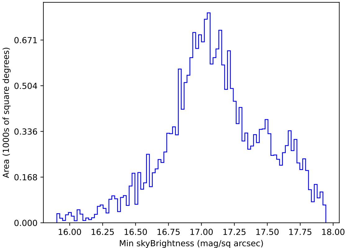
all_long_v3.4_10yrs All sky y band: Min skyBrightness
