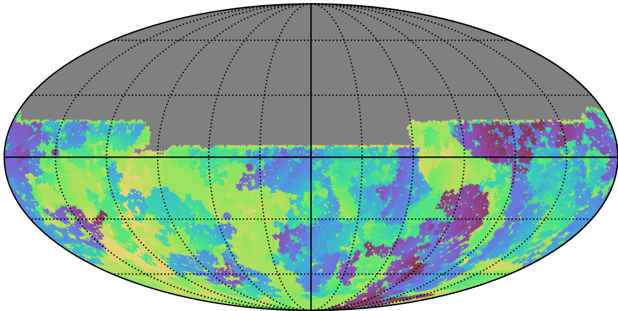
all_long_v3.4_10yrs All sky u band: Min skyBrightness
