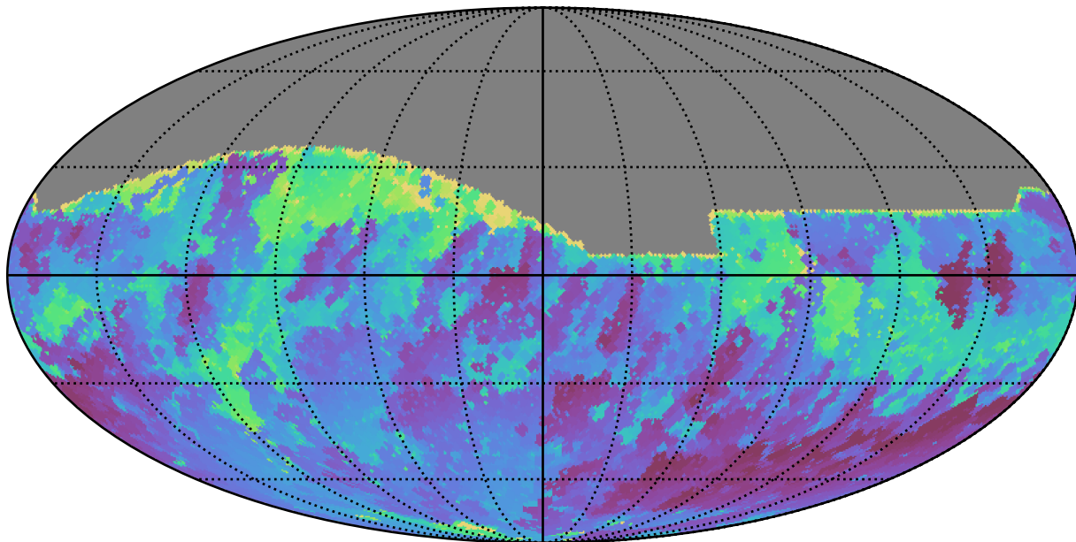
all_long_v3.4_10yrs All sky r band: Min skyBrightness
