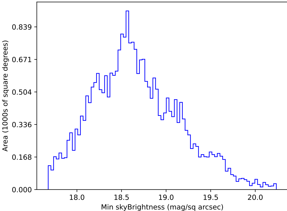
all_long_v3.4_10yrs All sky r band: Min skyBrightness
