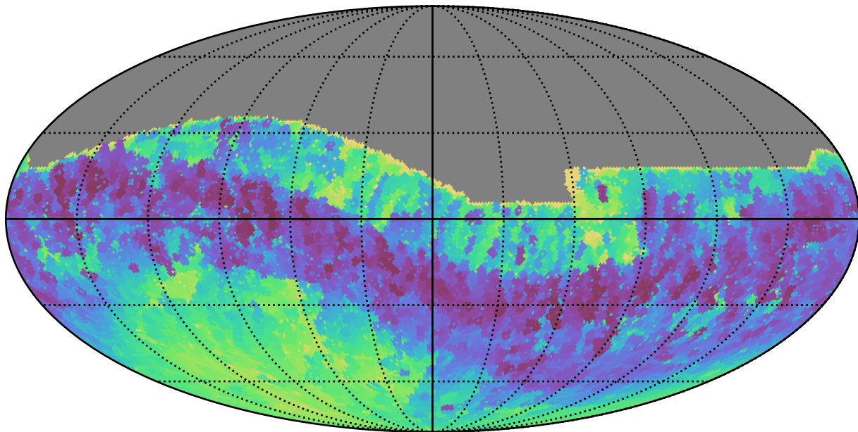
all_long_v3.4_10yrs All sky i band: Min skyBrightness
